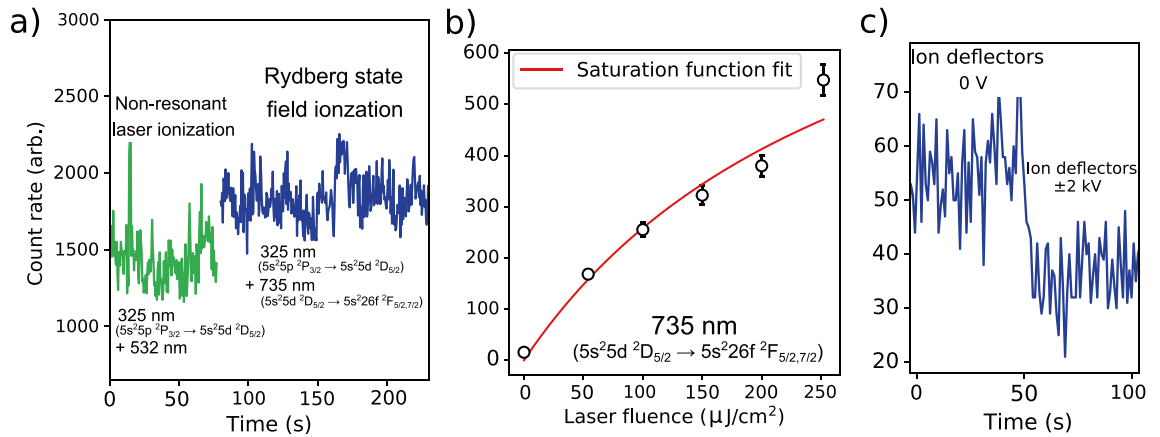
Figure 6. (a) The count rate on resonance for a typical non-resonant photoionization last step versus the field-ionization scheme corresponding to their total ionization efficiencies, (b) fitting the saturation curve 99 of the 5s^25d^2D_{3/2} \rightarrow 5s^226f^2F_{5/2,7/2} transition, giving a saturation fluence of 293(140) \mu\text{J}/\text{cm}^2 and (c) background rates with and without electrostatic deflectors to estimate background in the ‘interaction’ and ‘post-ionization’ region. Figure created using Refs. 44,45 .
