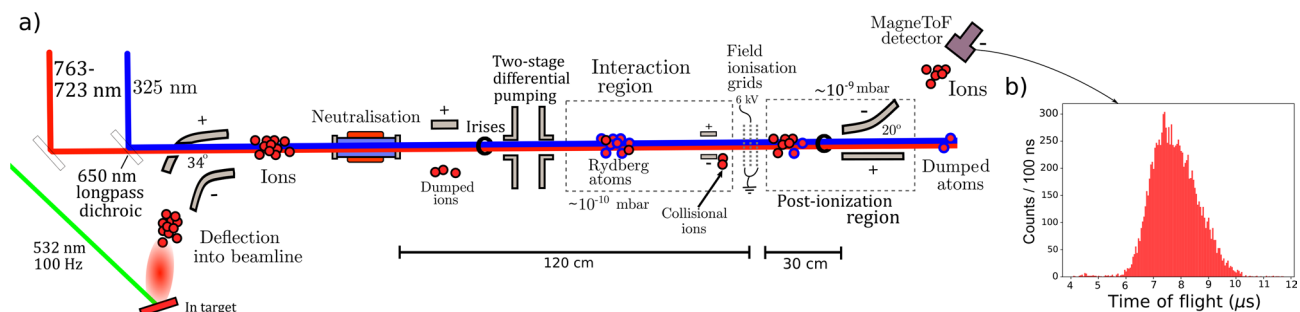
Figure 1. (a) A schematic diagram of the layout of the modified CRIS experiment, to use field ionization. Electrostatic deflectors guide the ions created by ablation to be neutralised. Atoms are excited to Rydberg states by a multi-step resonant laser scheme, and are subsequently field ionized and counted by an ion detector. (b) The time-of-flight distribution of the bunch created by the ablation ion source. Figure created using Refs. 44,45.
