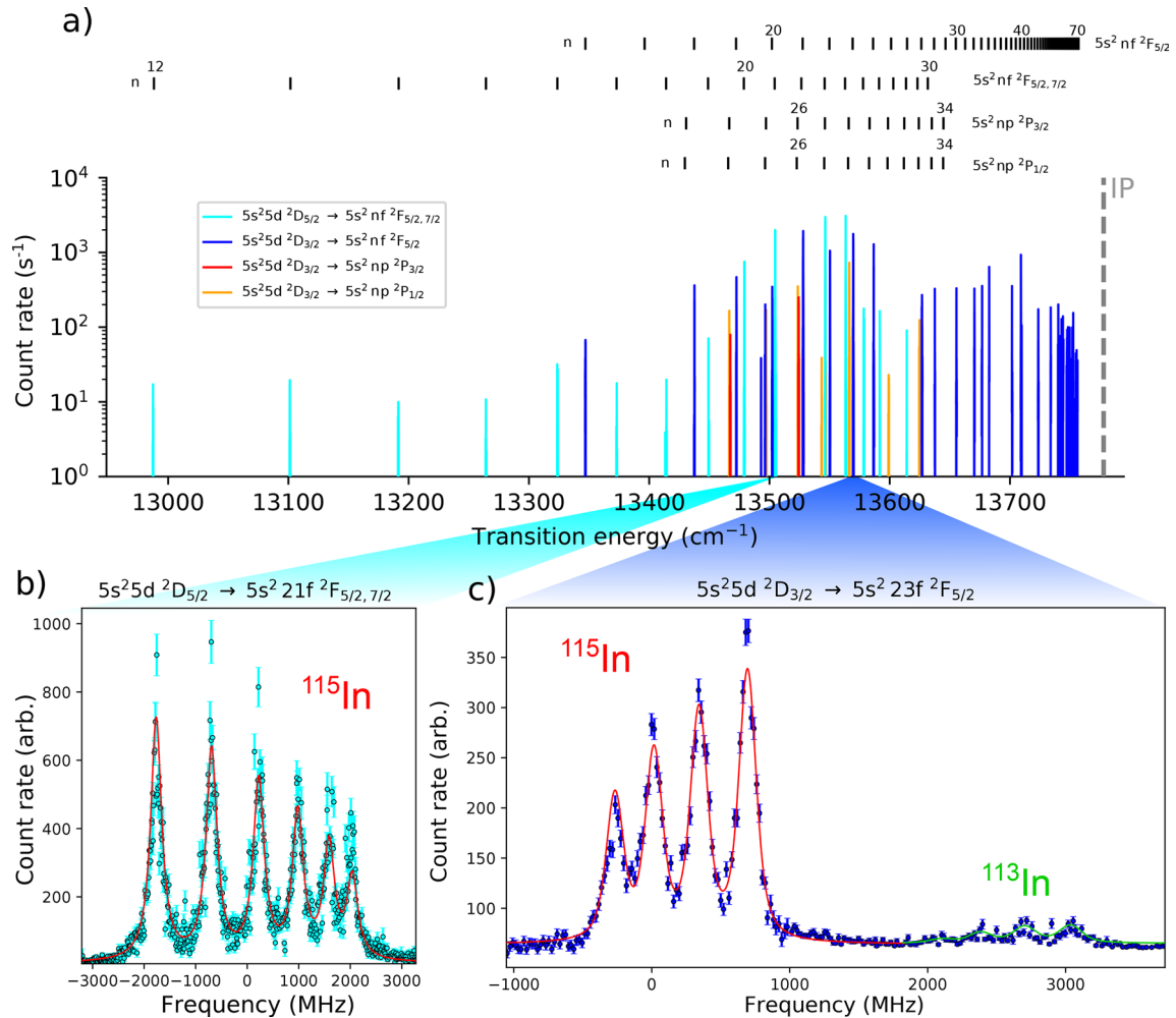
Figure 4. Summary of the high-resolution measurements of the transitions to Rydberg states from the {}^2P_{1/2} , 5s^2np , {}^2P_{3/2} , 5s^2np and {}^2F_{5/2} , 5s^2nf series, showing (a) the spectrum of resonances measured in the 770–720 nm range, with an inset in black indicating energies for the members of the Rydberg series using Expression 6. Example hyperfine spectra of the (b) 5s^25d \ ^2D_{5/2} and (c) 5s^25d \ ^2D_{3/2} lower states. Fits to the spectra of {}^{115}\text{In} are indicated in red. Figure created using Refs. 44,45 . A fit to {}^{113}\text{In} is indicated in green.
