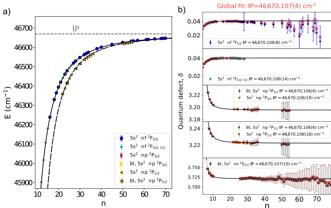
Figure 5. (a) Extracted energies of the 5s^2 np \ ^2P_{1/2} , 5s^2 np \ ^2P_{3/2} , 5s^2 nf \ ^2F_{5/2} and 5s^2 nf \ ^2F_{5/2,7/2} Rydberg series measurements. Literature values, labeled as 'lit', were taken from Ref. 60 . The black lines indicates the Rydberg expression values for the ^2F_{5/2,7/2} 5s^2 nf (solid line) and ^2P_{1/2,3/2} 5s^2 np series (dashed line). The ionization potential is indicated by the dashed grey line. (b) Determination of the ionization potential of the indium atom using a global simultaneous fit using Expressions 6 and 7 to \delta_n values of the 5s^2 nf \ ^2F_{5/2} , ^2P_{1/2,3/2} 5s^2 np , ^2P_{1/2,3/2} 5s^2 np and ^2P_{1/2,3/2} 5s^2 np of this work, along with literature ('lit') values for the ^2P_{1/2,3/2} 5s^2 np series 60 and ^2S_{1/2} 5s^2 ns 85 series. The red markers indicate series \delta_n values after the global fitting (IP = 46,670.107(4) \text{cm}^{-1} ). The IP value determined from the fit to each series independently are shown in their corresponding subplots. The black lines indicate series \delta_n values determined by Expression 7 from lowest-lying states 61 ( n = 4-10 for nf , n = 5-10 for np and n = 6-10 for ns ). Figure created using Refs. 44,45 .
